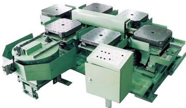
PALLET CHANGER
