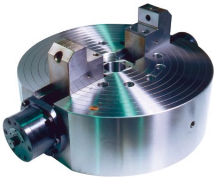
2 JAW FLOATINGCHUCK
