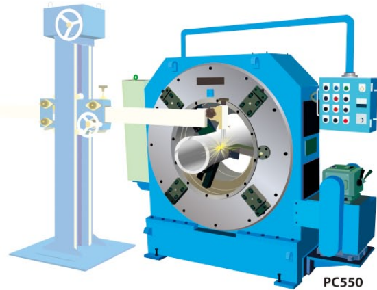
APPLICATION EXAMPLE
