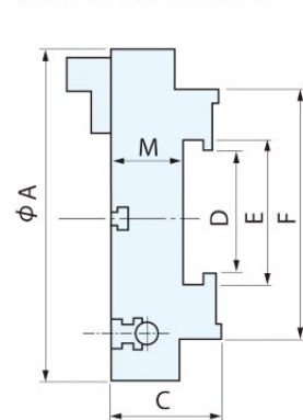
BORING MILL JAW PALLET
