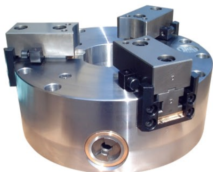
SPECIAL POWER WRENCH CHUCK \phi 400~ \phi 1800
